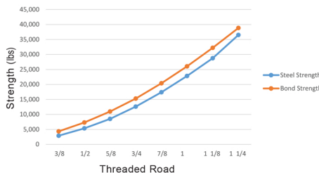
Grade 36 Threaded Rod, 10d Embedment Depth
