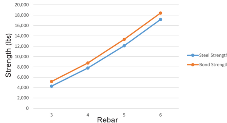
Grade 40 Rebar, 16d Embedment Depth
